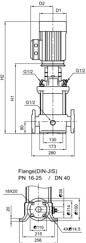
Version With Round Flanges PVM 10-14 - 10-20 PN16-25 / DN40
