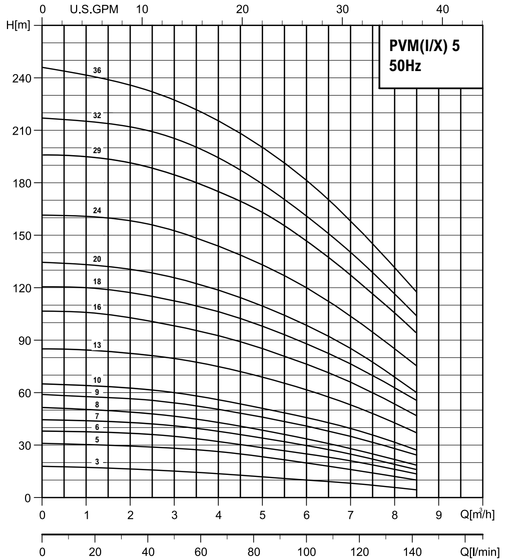
Version With Round Flanges PVM 5-24 - 5-36 PN25 / DN25/32
