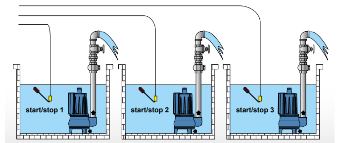
INSTALLATION EXAMPLES
