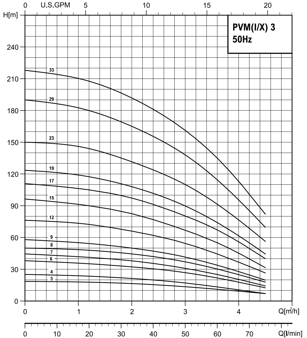
Version With Round Flanges PVM 3-23 - 3-33 PN25 / DN25/32
