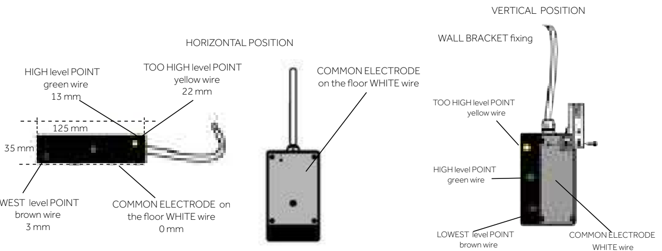
PUDDLE SENSOR
