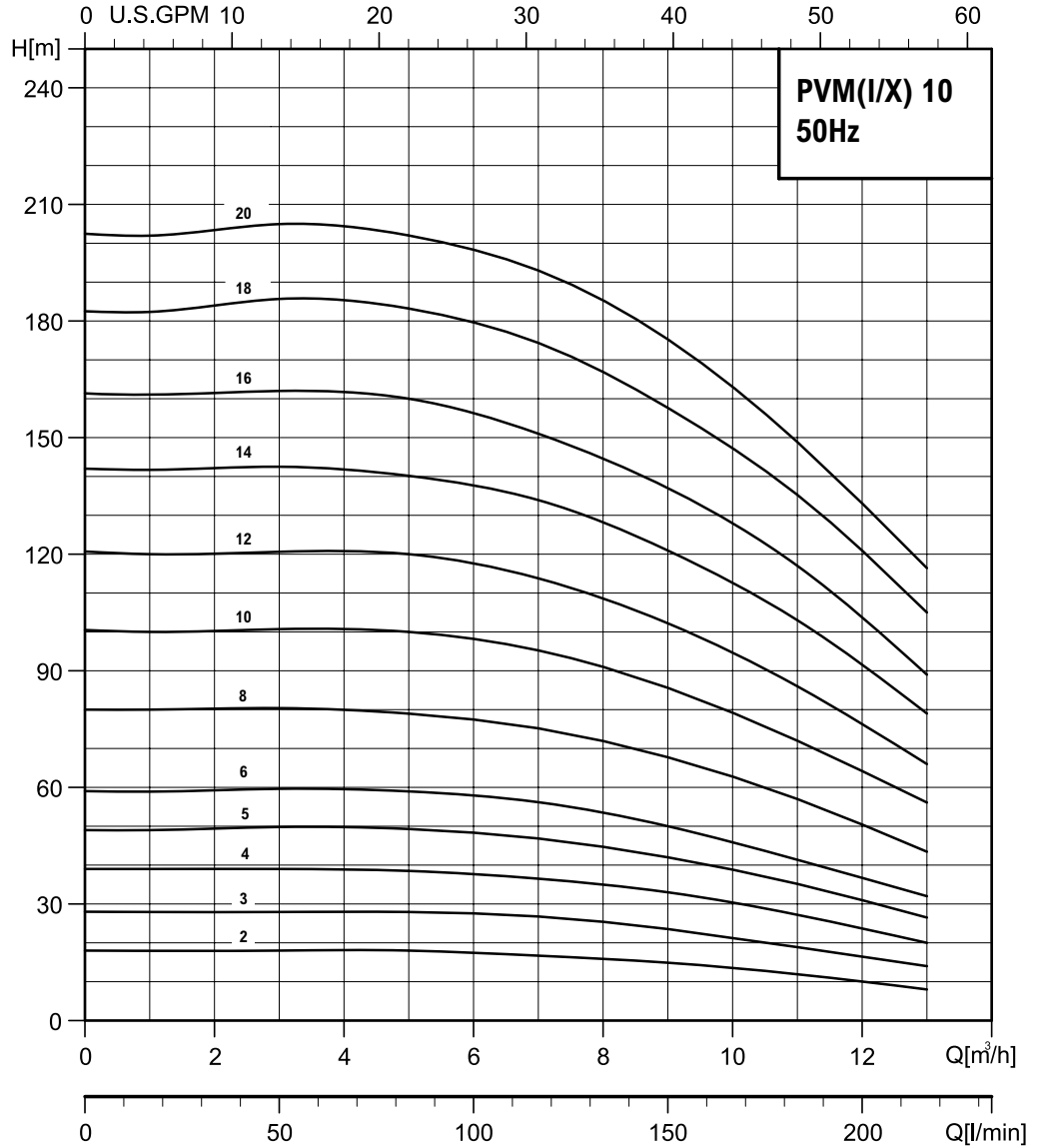
Version With Round Flanges PVM 10-14 - 10-20 PN16-25 / DN40
