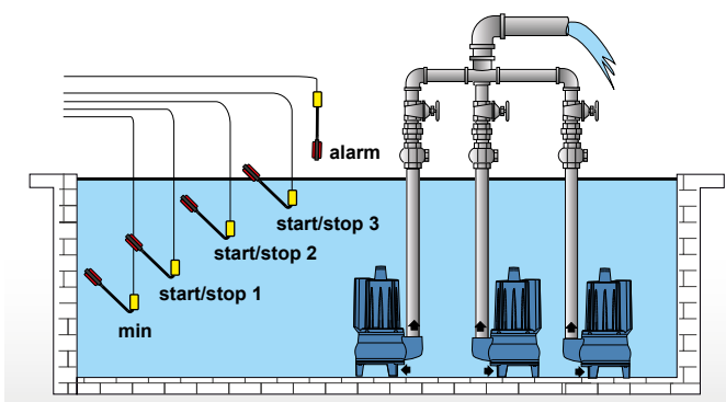
INSTALLATION EXAMPLES
