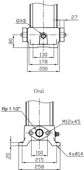
Version With Oval Flanges PVM 10-2 - 10-12
