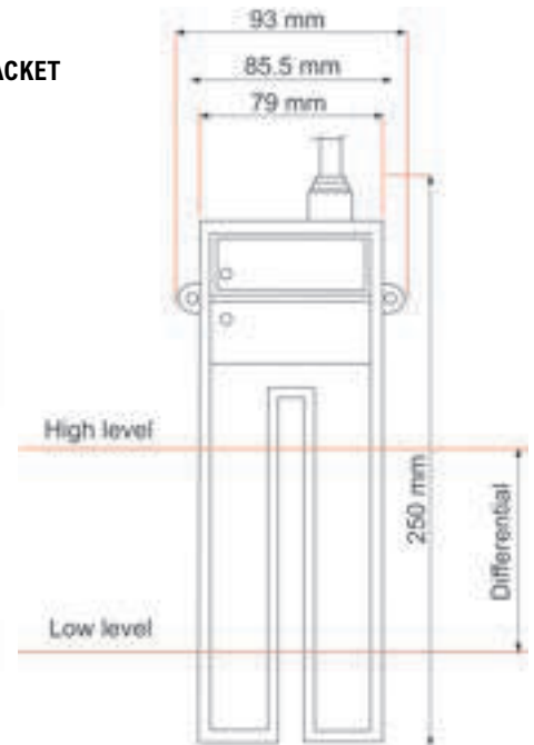
REKA C/W CABTYRE GLAND SHOWN ONTO JS150SV
