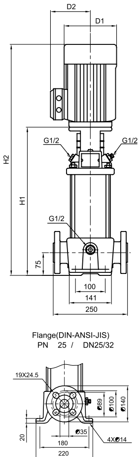
Version With Round Flanges PVM 3-23 - 3-33 PN25 / DN25/32
